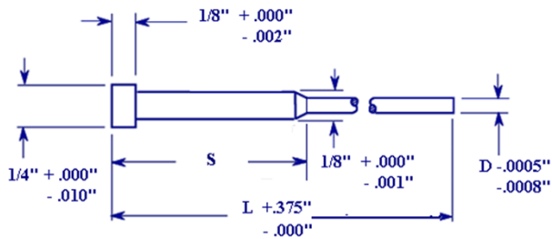
Shoulder Style Ejector Pin
