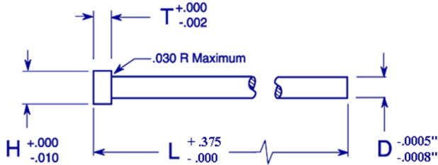
Straight Style Ejector Pins
